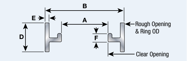
S-C Steel Deck Ring with Compression Seal
