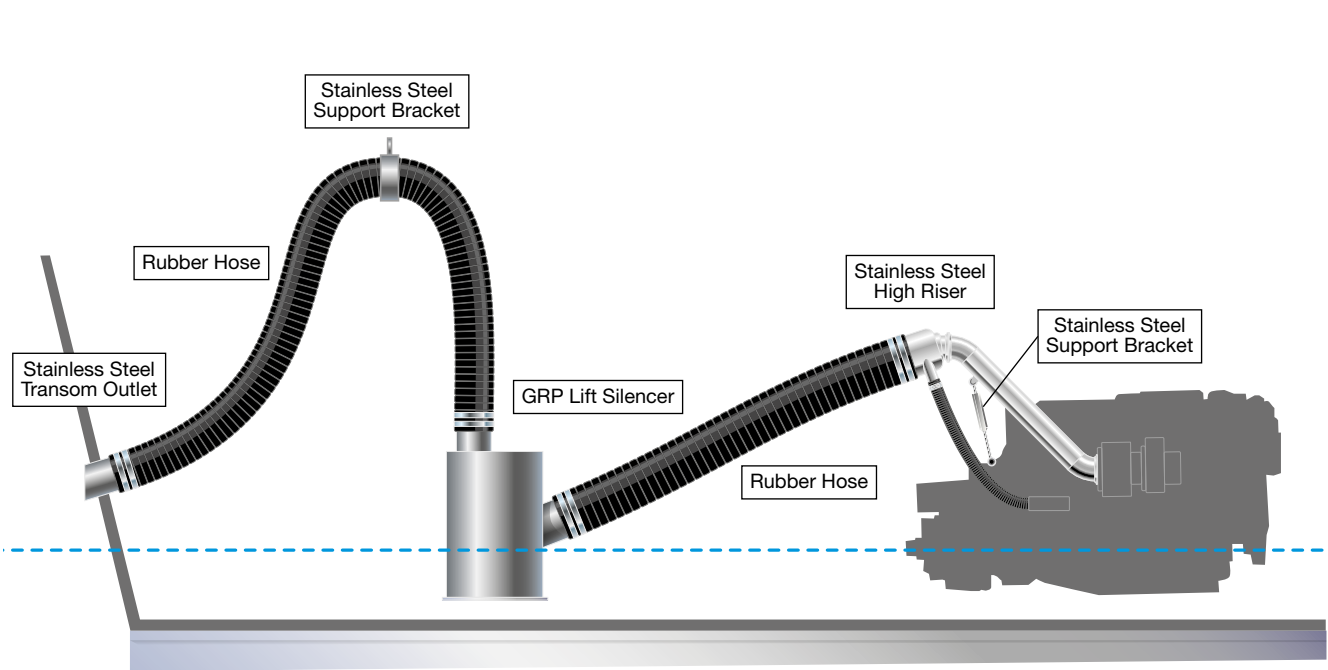
Example System - Single Chamber Lift Silencer with Discharge Above Waterline
