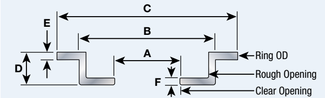
A-C Aluminium Deck Ring with Compression Seal
