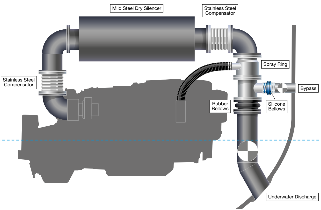
Example System - Dry Silencer to Spray Ring with Bypass & Underwater Discharge
