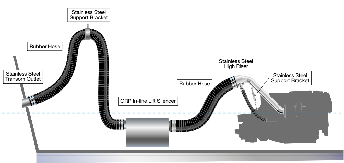
Example System - Standard In-line Lift Silencer with Discharge Above Waterline
