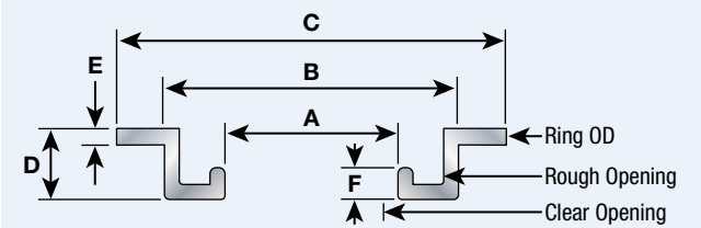
A-C Aluminium Deck Ring with Compression Seal
